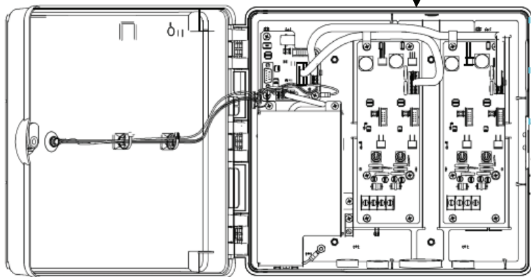
CONFIGURATION SHOWING TWO DRIVER BOARDS
